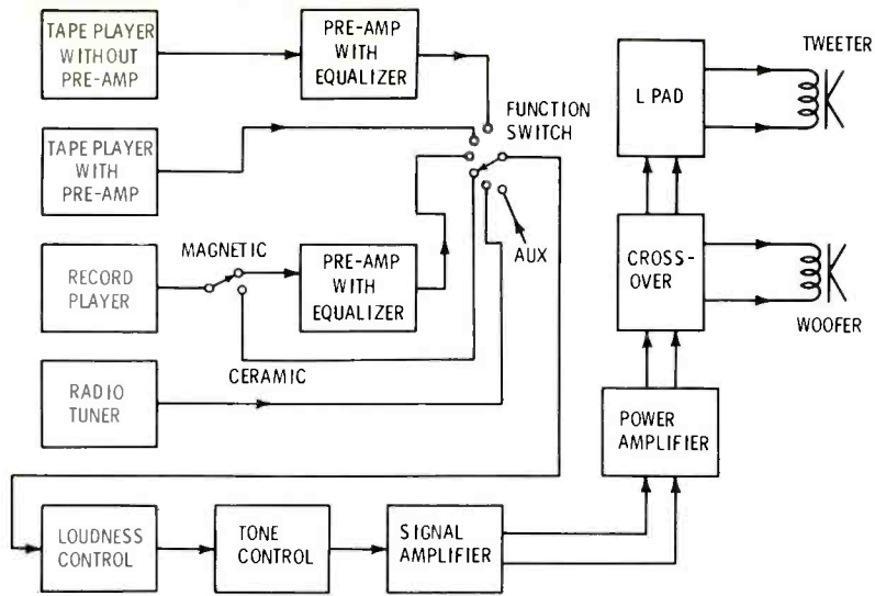
Fig. 1 Many modern stereo systems conform to this block diagram. The tape players, record changer, and radio must have two outputs for stereo; also two identical amplifiers and speakers are required.
