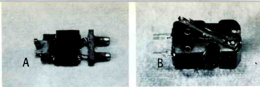
Picture (A) shows the inside of an old monaural crystal or ceramic phono cartridge. The stylus is supposed to be held in the groove of the rod at the left. An obsolete General Electric "variable reluctance" magnetic cartridge is pictured in (B). The dual-stylus assembly has been turned partially around to expose the two small pole pieces on the right. In this cartridge, the stylus moving between the pole pieces furnished the change of inductance.
