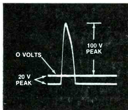
Fig. 4 A perfect series peak-reading rectifier should produce +100 volts from this waveform. Of course, that's the same as the voltage of the positive peak. Also, a perfect series peak-reading rectifier should produce -20 volts from the same waveform, by rectification of the 20-volt negative peak. Figure 3 showed how a heavy load can reduce the output voltage, and the article explains the effects of the different conduction times when the two peaks are rectified. In practice, a pulse rectifier might produce a DC output of 70% of the p-p input, if lightly loaded, or a heavy load might reduce that to 30%. Scan supplies might produce from 20% to 10%, depending on loading.
