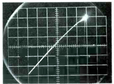
Fig. 4 A NORMAL/INSTA-BETA DISPLAY switch gives the choice of a family of curves or the single diagonal line of Insta Beta. The waveform is the Insta Beta display of a non-defective PNP germanium audio-type transistor, having a gain of about 90.
