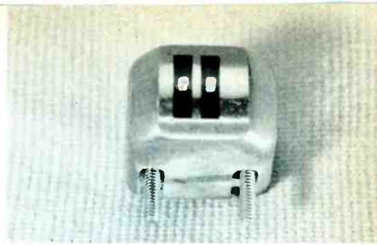
This tape head is for four tracks on 1/4-inch tape.
