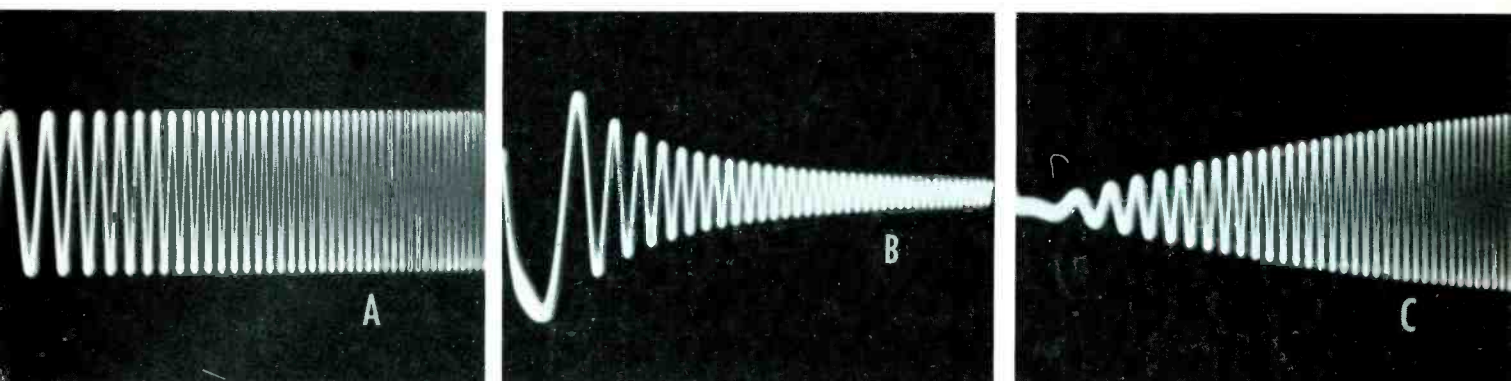
Fig. 4 (A) The waveform is an audio tone swept from a low frequency at the left to a higher frequency at the right. This is "constant-amplitude" response, in which the amplitude is the same for all frequencies. (B) "Constant-velocity" response increases the amplitude at low frequencies. (C) The decrease of low frequencies shown here could be caused by playing a constant-amplitude recording with an unequalized magnetic cartridge. Note: these waveforms were produced by sweeping the audio-frequency sine waves of a Tektronix FG502 function generator by the sawtooth output of a Hickok function generator.
