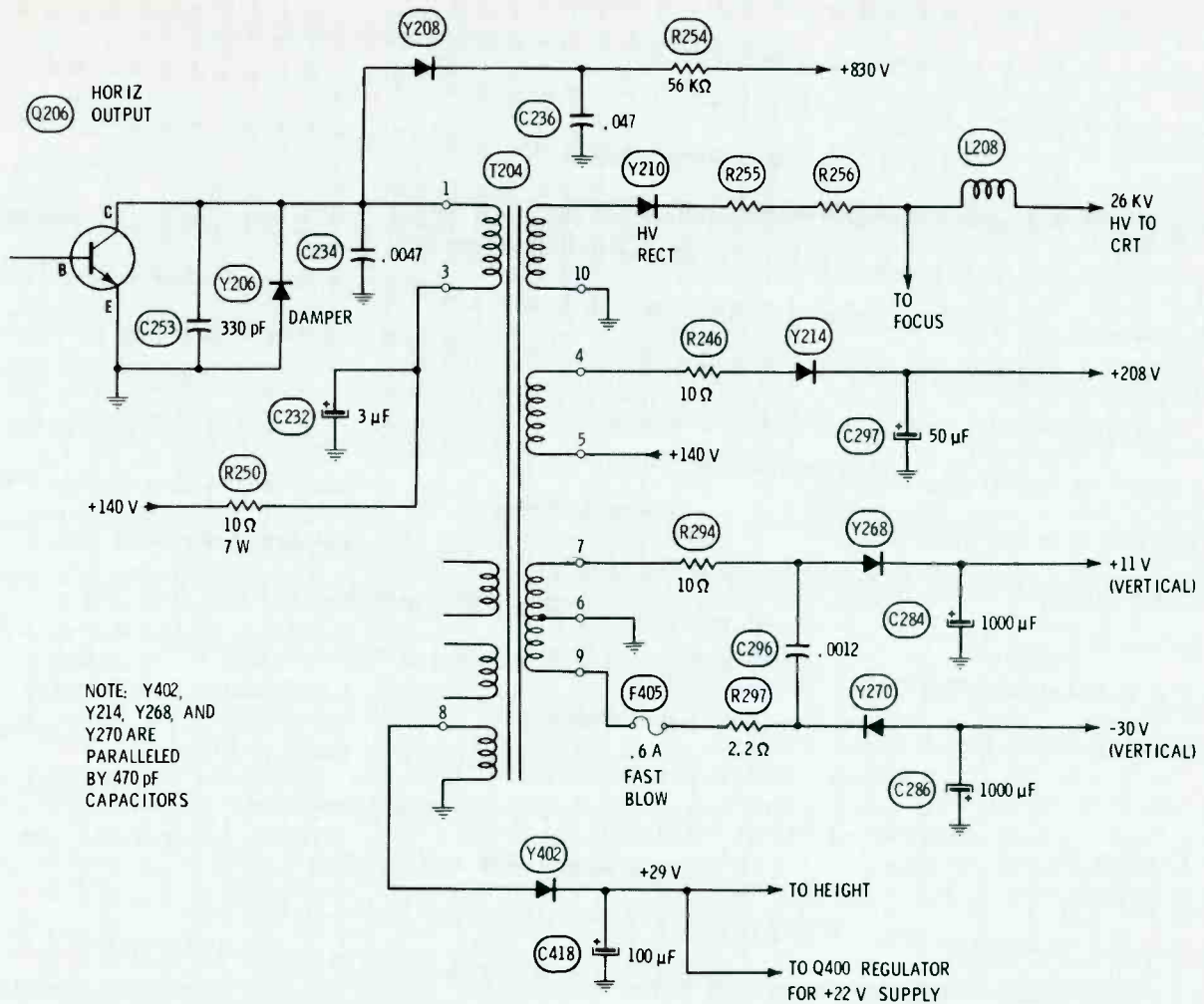
Fig. 6 The General Electric 19FA chassis has one pulse-rectifier supply and four scan-rectifier supplies. Y268 and Y270 diodes are on the vertical module, so if there's a doubt that excessive vertical current is blowing the fuse or reducing the high voltage, the module can be unplugged as a test.
