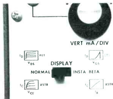
Fig. 4 A NORMAL/INSTA-BETA DISPLAY switch gives the choice of a family of curves or the single diagonal line of Insta Beta. The waveform is the Insta Beta display of a non-defective PNP germanium audio-type transistor, having a gain of about 90.
