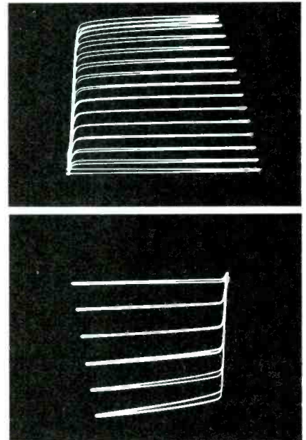
Fig. 3 Base current per curve is selected by the BASE GENERATOR switch, and the number of curves is determined by the setting of STEPS/FAMILY SWEEP LENGTH control. The control is continuously adjustable, but the curves pop in or out with a complete one each time. The waveform with 14 curves plus the base line is from a silicon NPN low-gain transistor, while the other with five curves plus the base line represents a medium-gain germanium PNP transistor.
