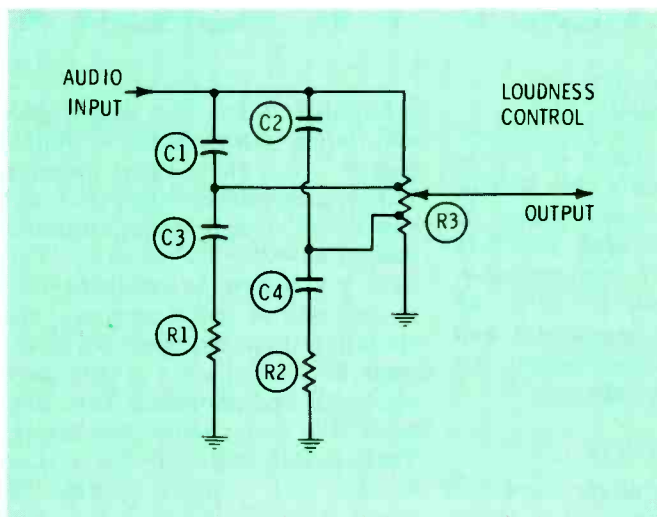
Fig. 6 This type of loudness-control circuit boosts both bass and treble as the volume is reduced, partially compensating for the Fletcher-Munson effect.
