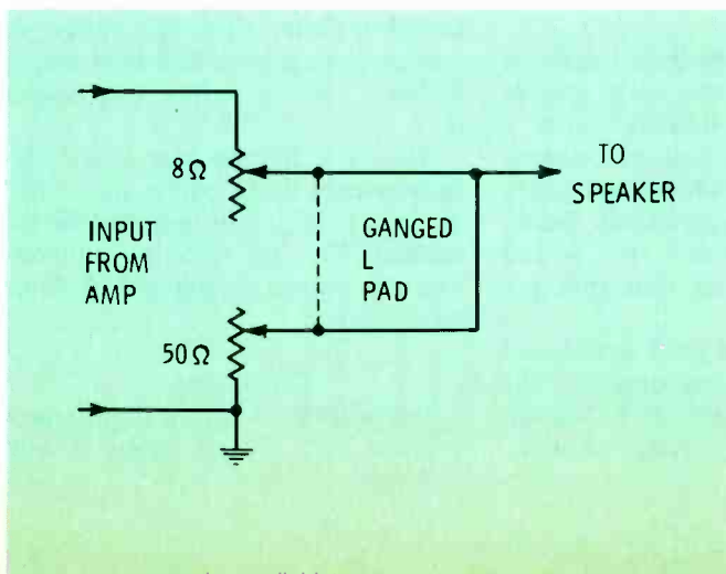
Fig. 7 "L" pads that adjust the volume applied to a speaker usually have two separate resistive elements. The circuit avoids loading the amplifier, and maintains constant input impedance at all levels, which a simple pot cannot do.
