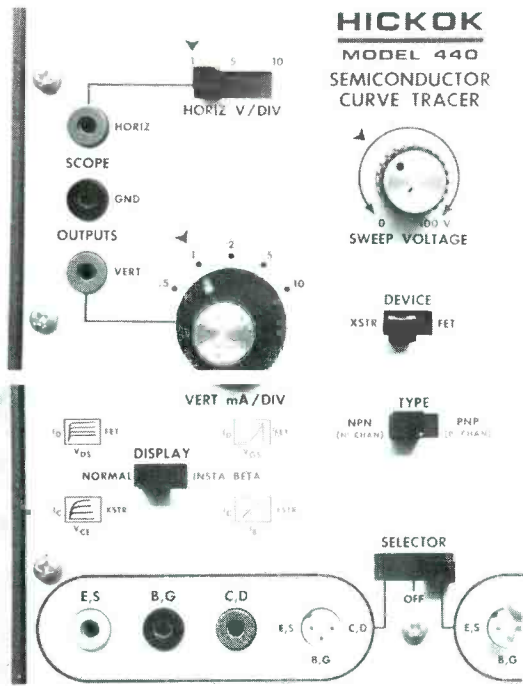
Fig. 1 The clearly-labeled banana jacks for connecting to the scope are located conveniently on the panel, along with the attenuation switches. The switches permit changing the size of the display, without upsetting the scope gain calibrations.
