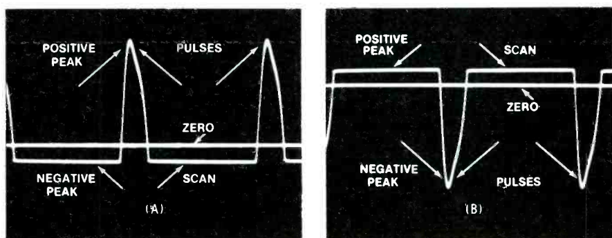
Fig. 1 A diode rectifier operates on the voltage between the appropriate peak and the zero point of the AC input voltage. The amount of DC voltage obtained from rectifying pulses, such as the ones from horizontal sweep, depends on which peak is rectified. Rectification of the positive peak of "A" would produce a much larger positive voltage than would rectification of the positive peak of "B". In the same way, the negative peak of "A" would yield a low negative DC voltage, and the negative peak of "B" would produce a larger negative DC voltage after rectification. In practice, the ratio of the DC voltages obtained from the two peaks varies between three times and five times, depending on the width of the pulses and the load on the supply.
