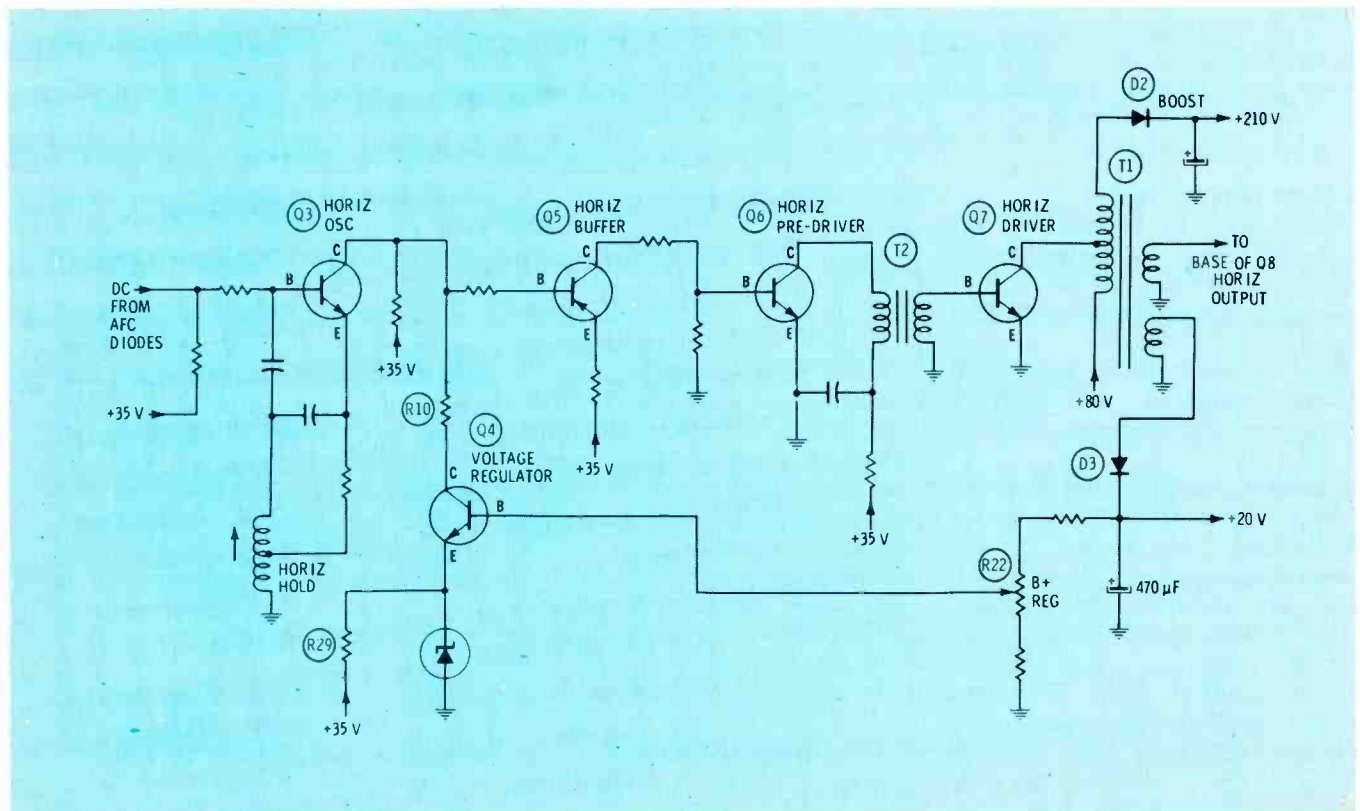
Fig. 7 Two sweep-rectified supplies are found in the Quasar TS941 chassis, but the AC comes from the horizontal-driver transformer, not from the flyback.
