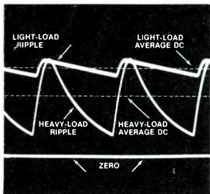
Fig. 3 Examine this multiple-exposure waveform carefully; it's probably the first time it has ever been published. Shown here are the DC voltages and ripple waveforms of a certain peak-
