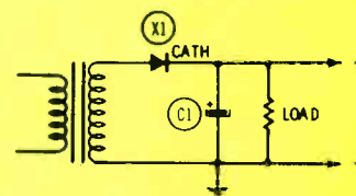
Fig. 2 This half-wave peak-reading rectifier circuit is a series type, with the correct diode polarity for rectification of the positive peak, which will produce positive DC at the load. For rectification of the negative peak, just reverse the polarity of the diode, and the output then will be negative DC.
