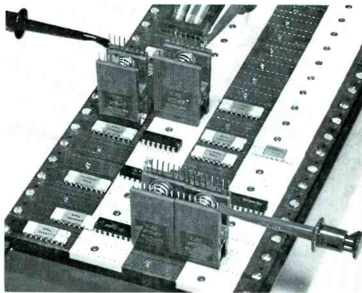
Original wide body DIP CLIP shown at rear for size comparison.
