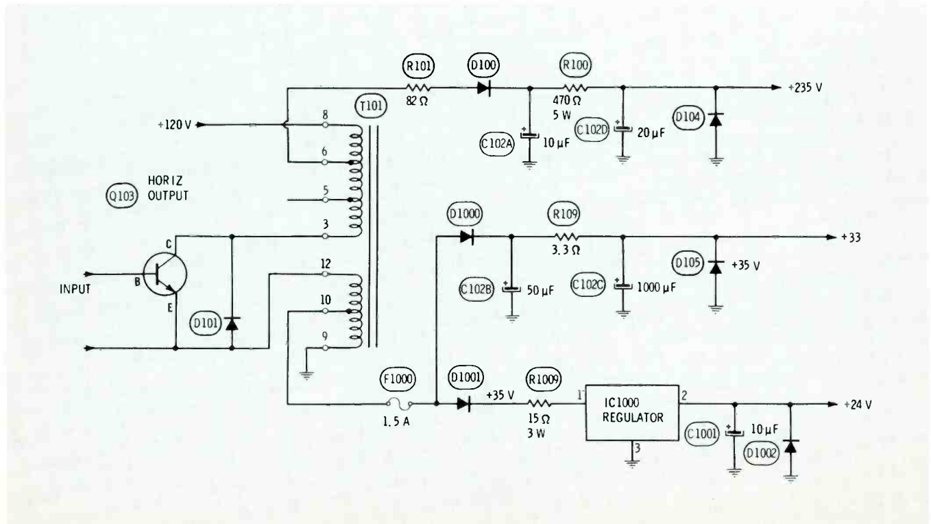
Fig. 5 Three pulse-rectified supplies are used in the Admiral M10 chassis. Notice that the +235 voltage is made up of +120 volts from the DC supply to the horizontal-output transistor plus about +115 volts from pulse rectification. An open F1000 fuse causes loss of vertical sweep and no sound, except for some buzz.
